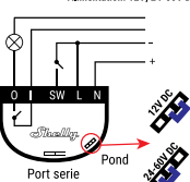
fig.2 Alimentation: 12V; 24-60V DC
